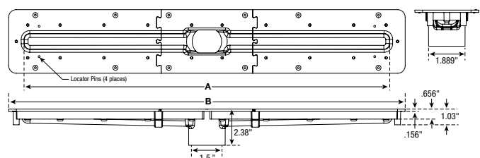
DIMENSIONS (1-1/2" VERTICAL WASTE OUTLET)
