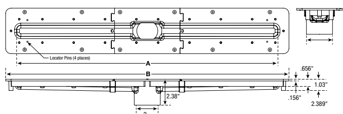
DIMENSIONS (2" VERTICAL WASTE OUTLET)
