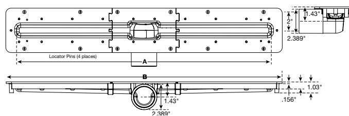
DIMENSIONS (2" SIDE WASTE OUTLET)
